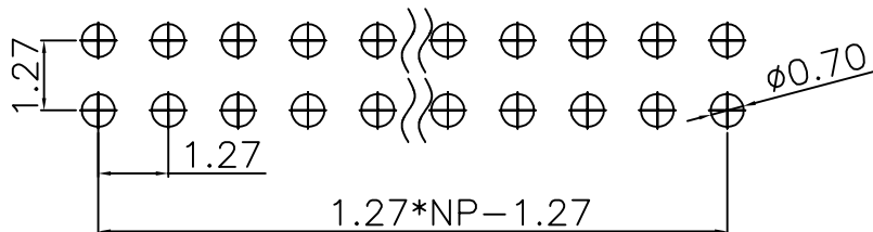
PCB LAYOUT
